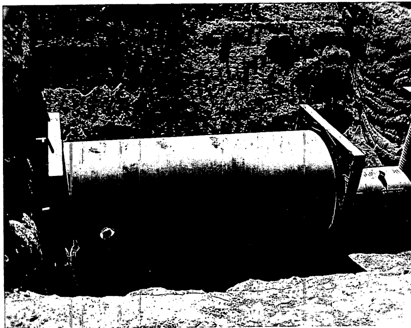
Fig. 7—Exterior view of typical circular concrete conduit before backfilling.
